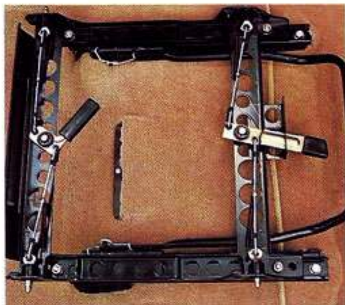
Volvo's front seat frame, securely anchored at four points.
