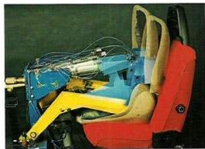
Volvo's reputation for toughness isn't just because of thick paint. Volvo also invests heavily in sophisticated testing and quality-control equipment and procedures. This machine, for instance, can put years of stress and wear on a seat in a matter of days. It represents Volvo's dedication to quality.
