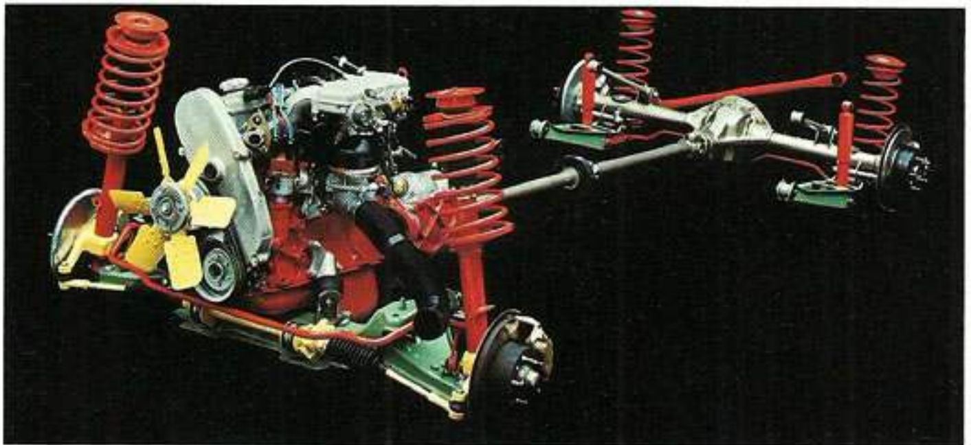
Volvo 240 and 260 Series cars ride on a front suspension with McPherson struts, coil springs, internal shock absorbers, stabilizer bar and rack-and-pinion steering.
