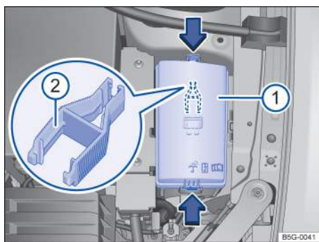
Fig. 157 In the engine compartment: Fuse box cover ① with tweezers ② .
