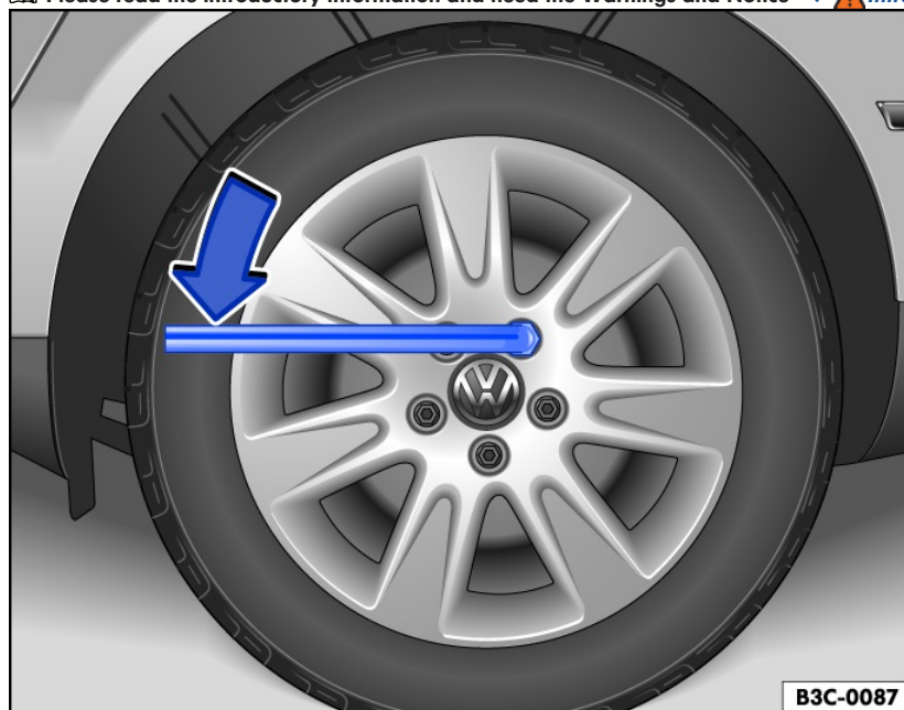
Fig. 169 Changing a tire: loosening the wheel bolts.
