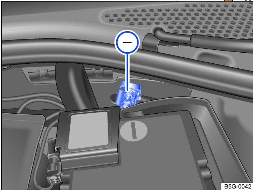
Fig. 142 In the engine compartment: jump-start point (negative connection).
