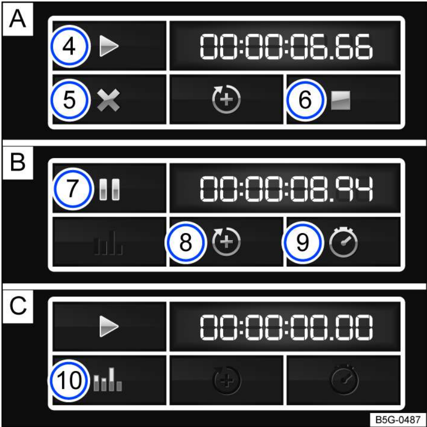
Fig. 20 Function key on the Infotainment system screen: time measurement when the lap is A stopped, B running, and C finished.
