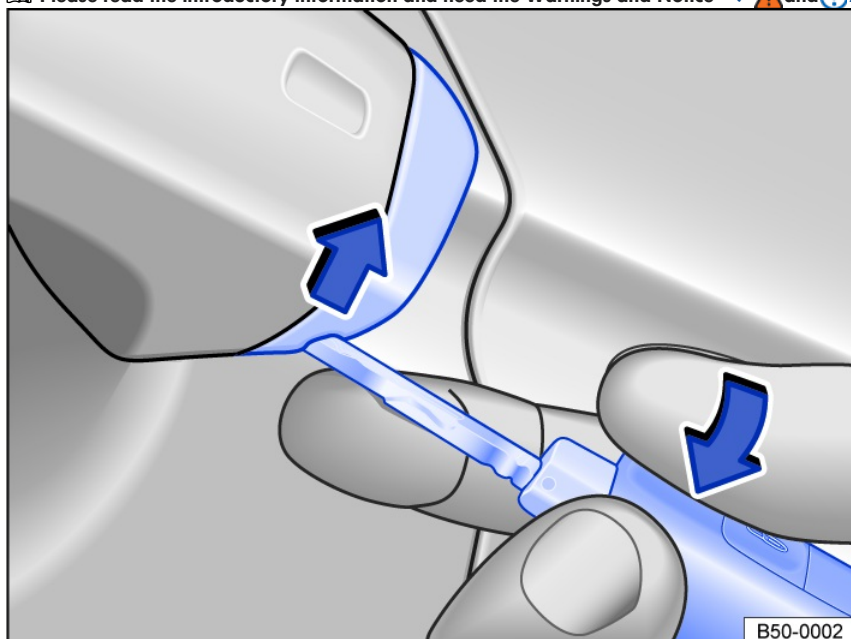
Fig. 57 Driver's door handle: prying off the cap.
