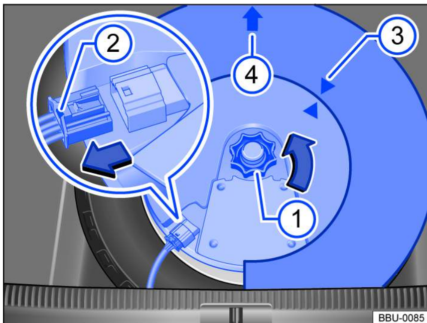
Fig. 171 In the luggage compartment: removing the subwoofer (version 2).
