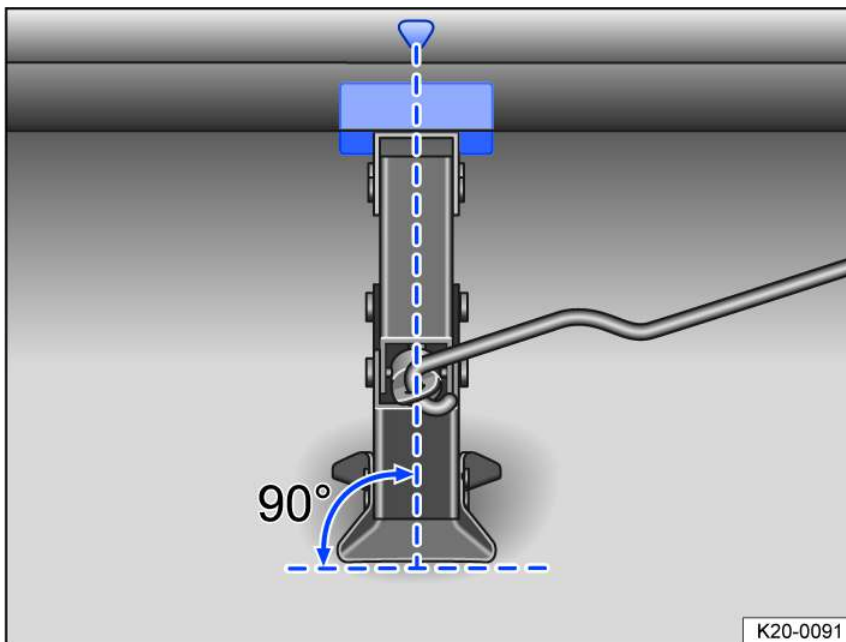
Fig. 174 Correct jack setup.
