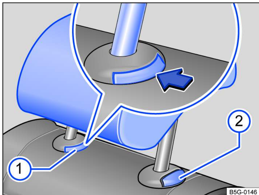
Fig. 75 Rear head restraint: removing.
