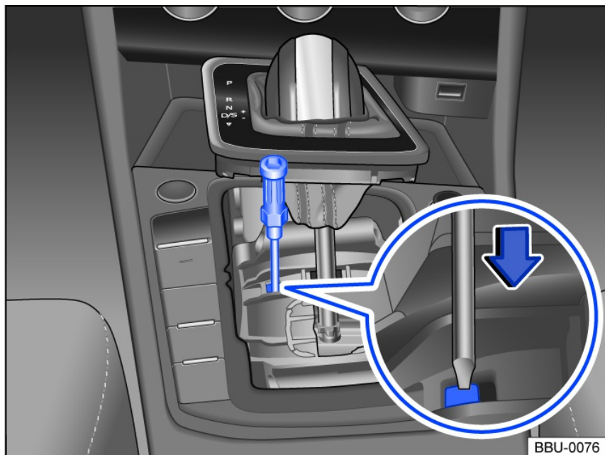
Fig. 105 Manually release the selector lever lock.
