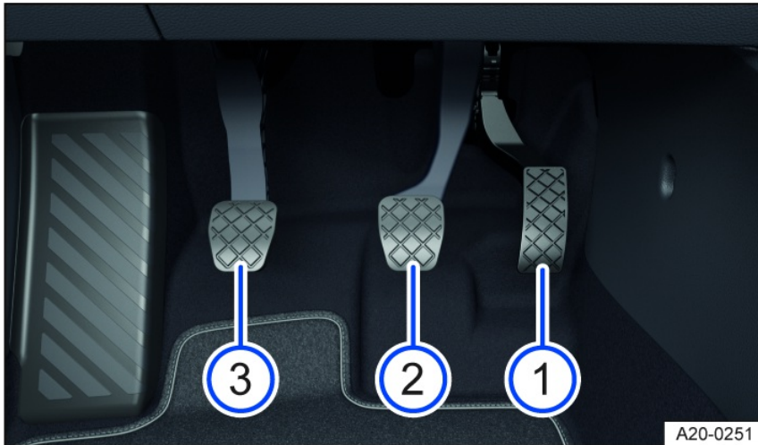
Fig. 90 In the footwell: Pedals in vehicles with a manual gearbox.
