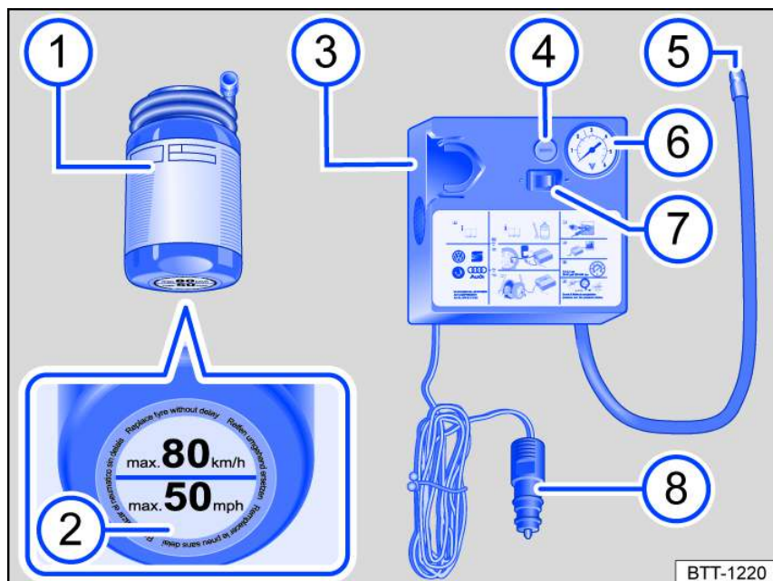
Fig. 180 General example: components of the tire mobility set.
