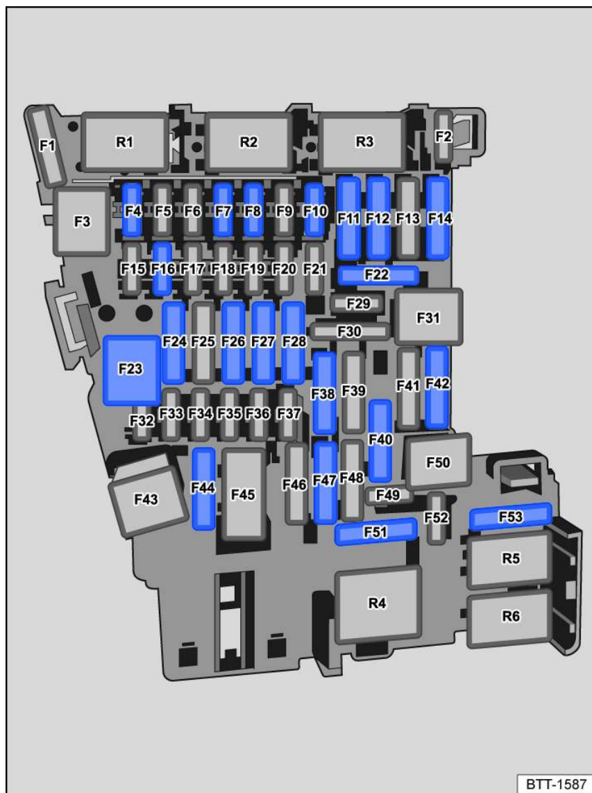
Fig. 139 Fuse assignment in the instrument panel.
