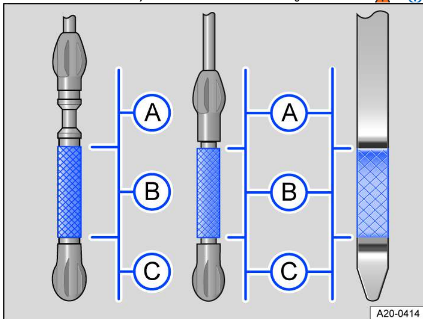
Fig. 154 Engine oil level markings on the oil dipstick (versions).
