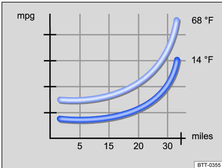
Fig. 93 Fuel consumption in mpg at two different ambient temperatures.
