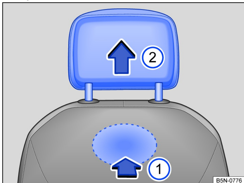
Fig. 74 Front head restraints: removing.
