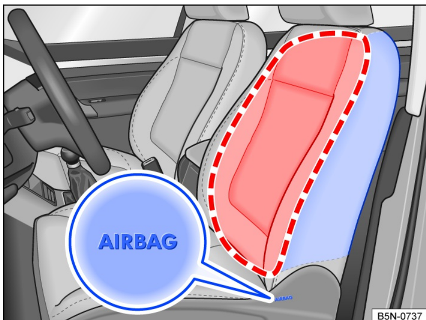
Fig. 37 On the side of the front seat: Side airbag installation location and deployment zone
