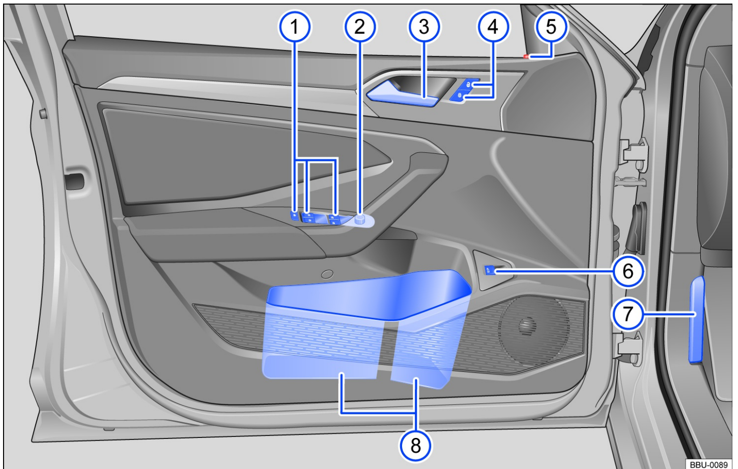
Fig. 6 Driver door: Controls.
