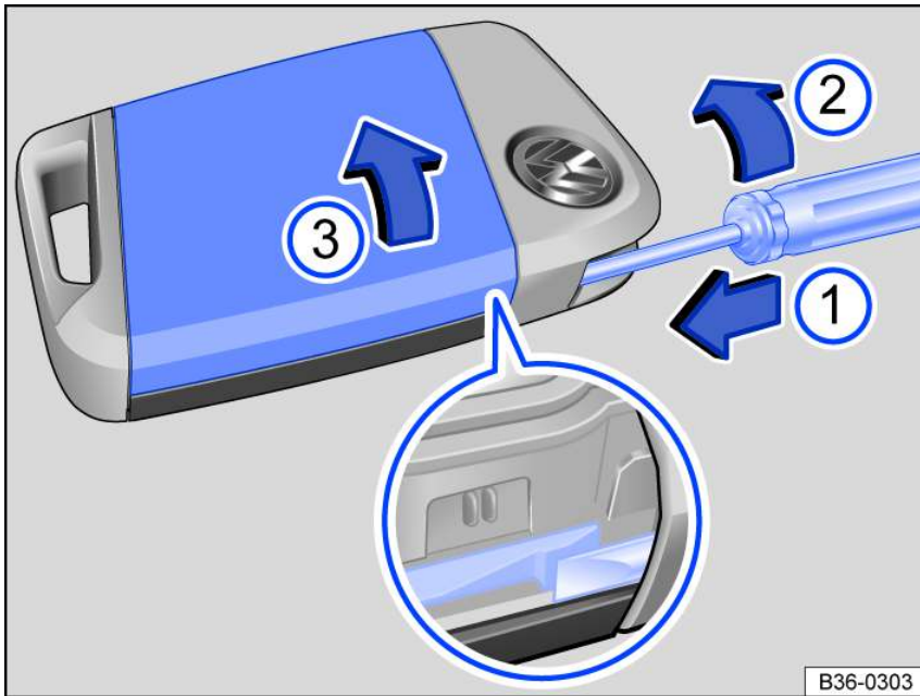
Fig. 52 Vehicle key: opening the battery compartment cover.
