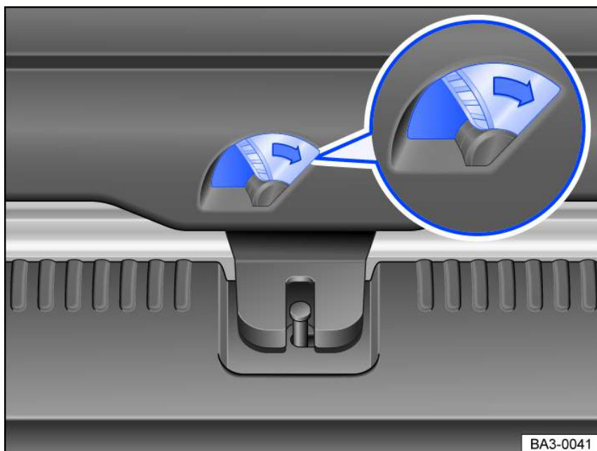
Fig. 63 In the luggage compartment: mechanically unlocking the trunk lid using the emergency release.
