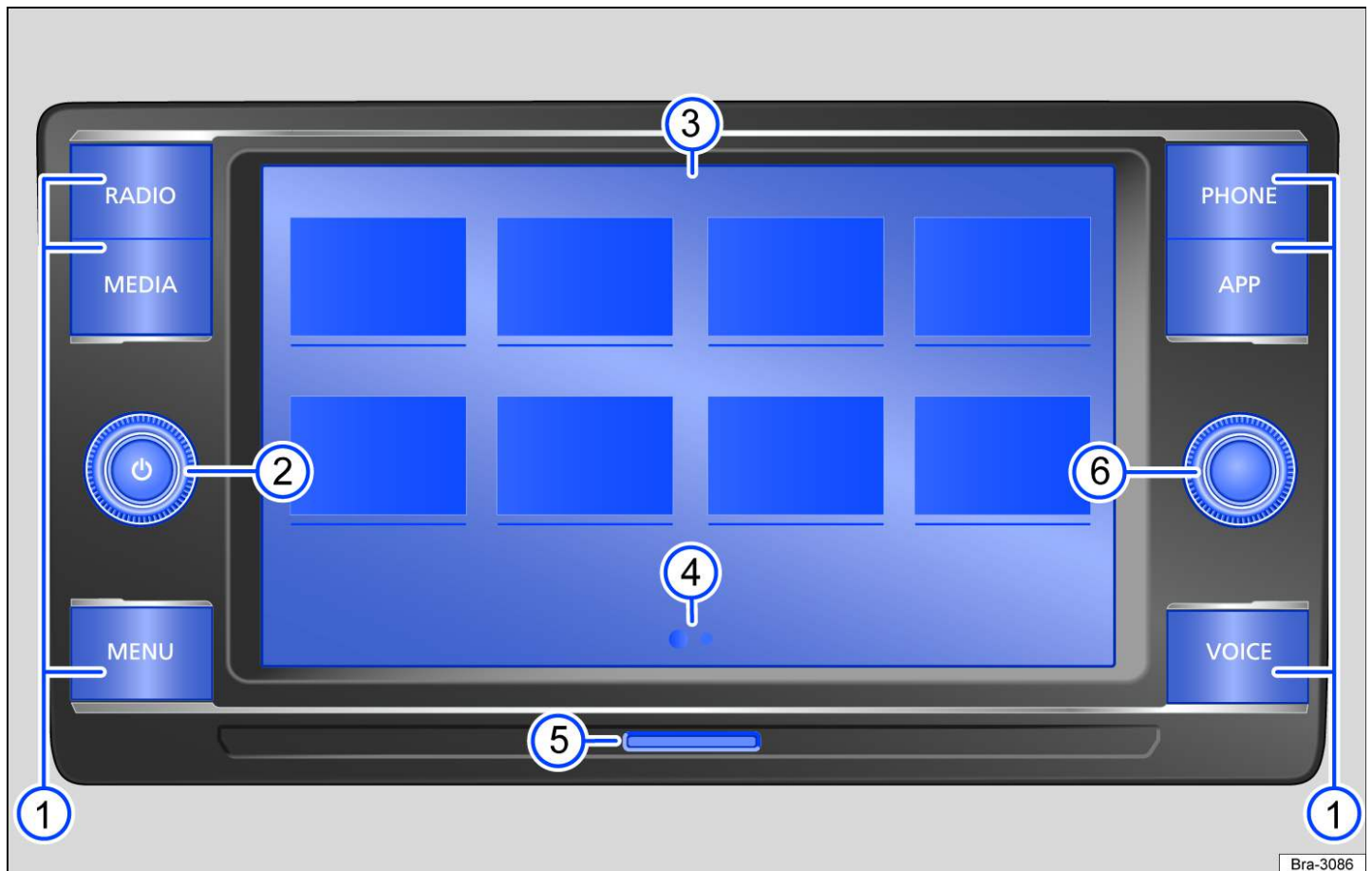
Fig. 125 Overview: Radio in the 6.5 inch variant (6.5").
