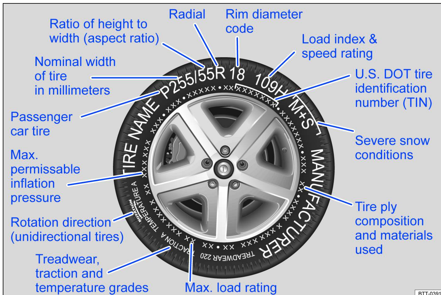
Fig. 164 International tire labeling.
