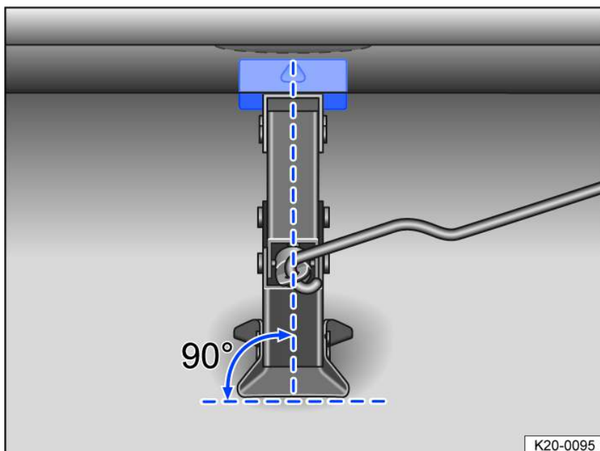
Fig. 177 Correct jack setup.
