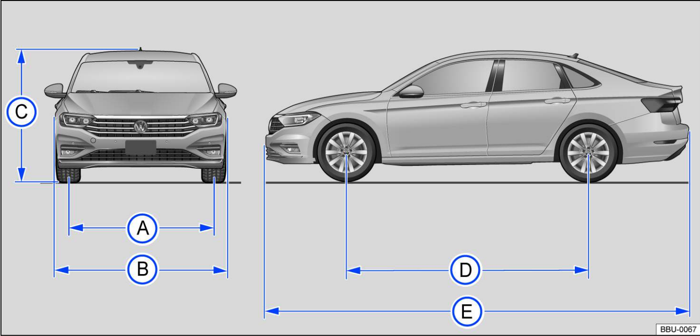
Fig. 188 Vehicle dimensions.
