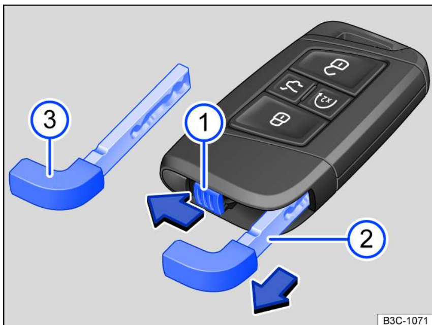
Fig. 51 Vehicle key: releasing the emergency key.
