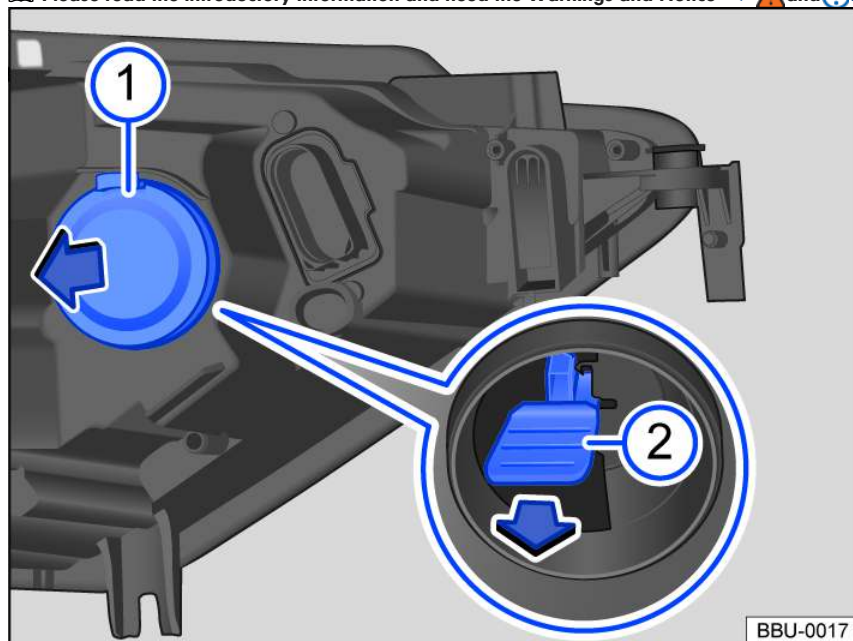
Fig. 135 In the right-side of the engine compartment: Rear side of the headlights.
