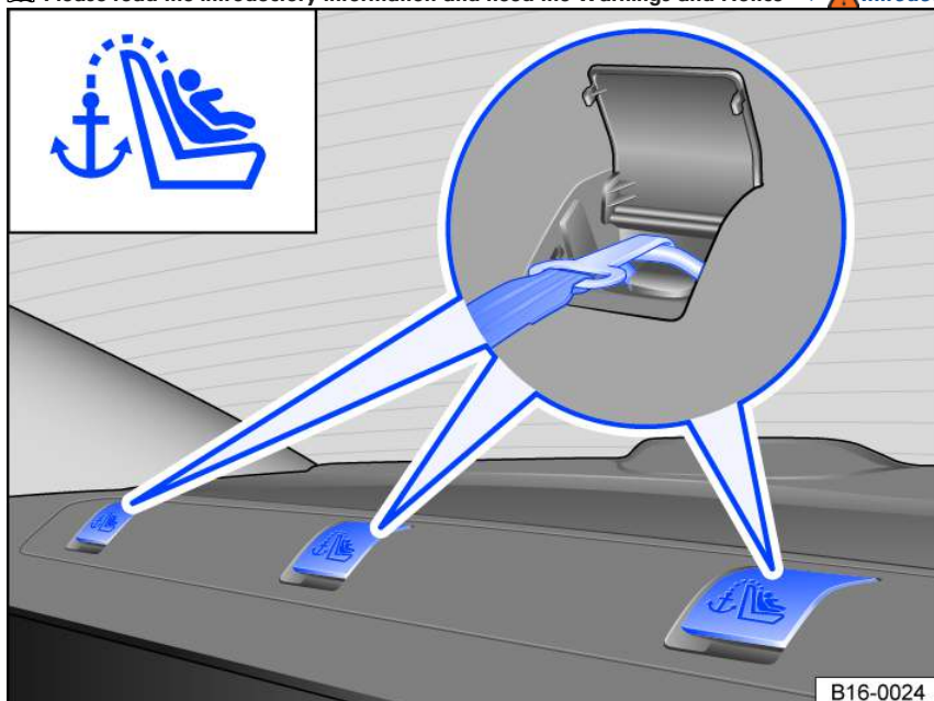
Fig. 42 In the storage compartment behind the rear bench seat: Anchorages for the upper strap.
