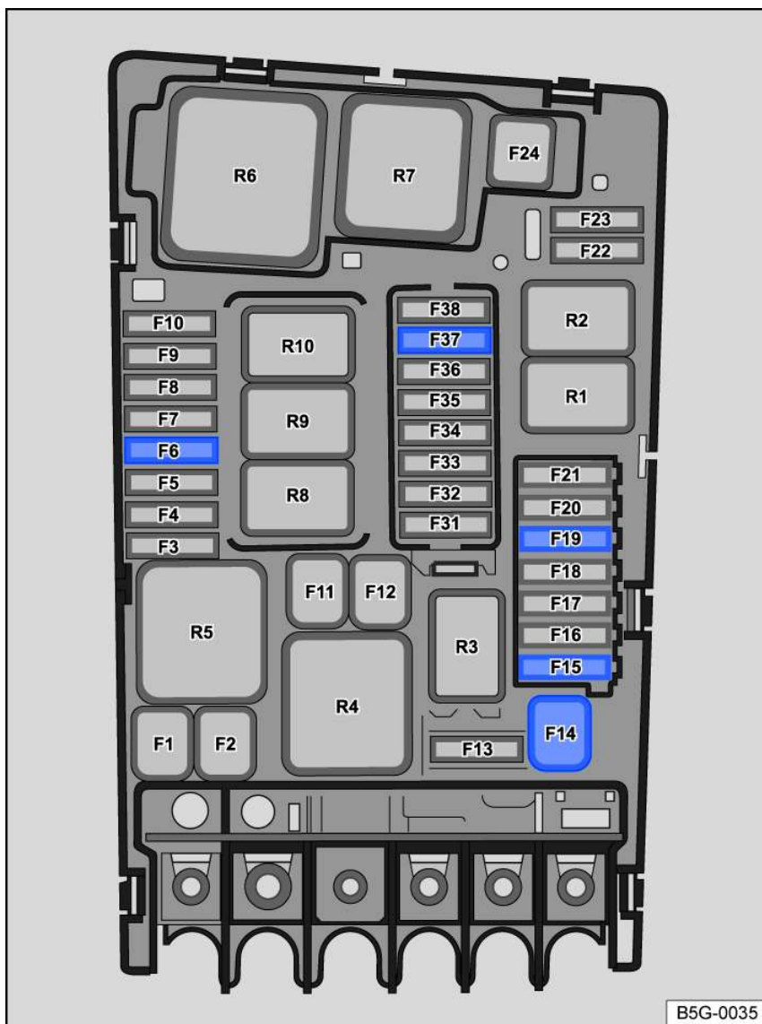
Fig. 137 Fuse locations in the engine compartment.
