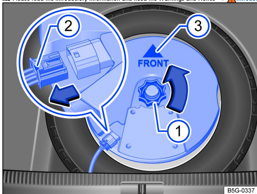
Fig. 170 In the luggage compartment: removing the subwoofer (version 1).
