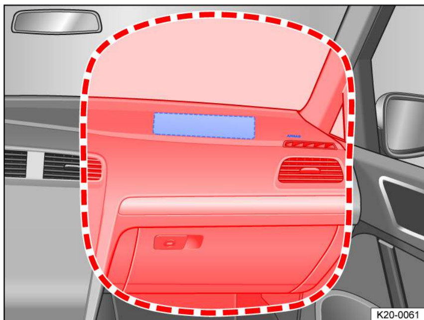
Fig. 35 Installation location and deployment zone of the front passenger's front airbag.
