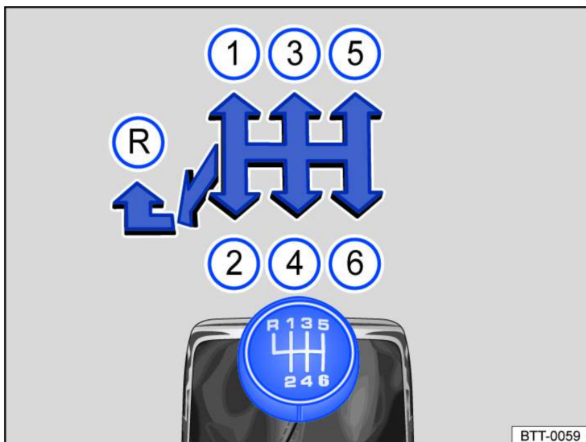
Fig. 100 Gear shift pattern for 6-speed manual transmission.
