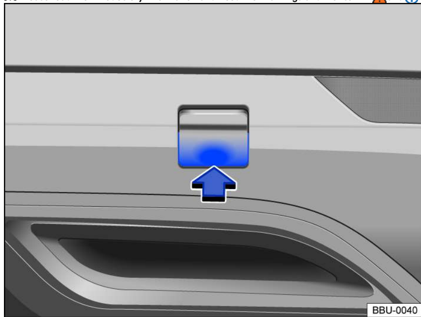
Fig. 146 In the right rear bumper: Cover for the towing eye mount.
