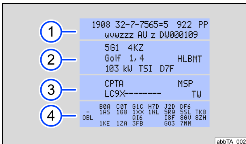
Fig. 187 General example: vehicle data label.
