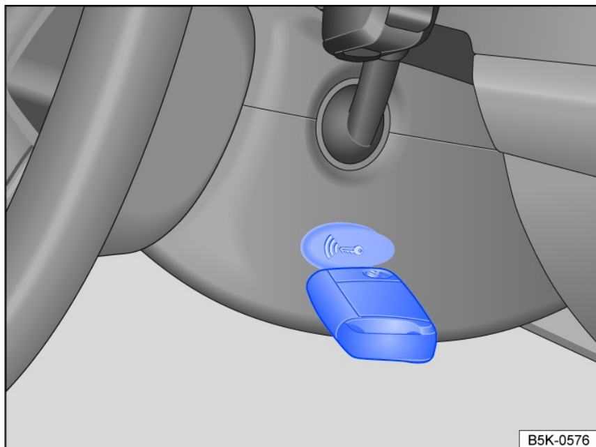
Fig. 98 On the right side of the steering column: emergency start function on vehicles with Keyless Access with push-button start.
