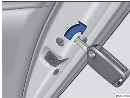
Fig. 56 On the front side of the rear passenger door: Locking the vehicle with the key bit in the vehicle key.
