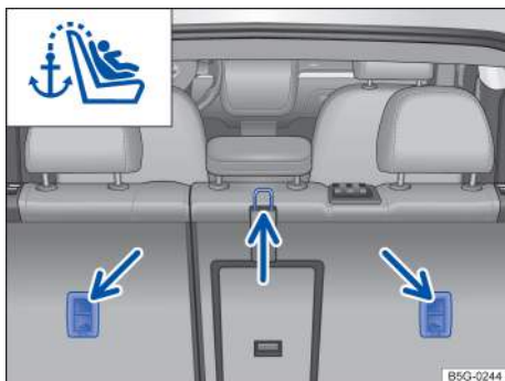
Fig. 46 Anchorages for the top tether strap on the back of the rear seat.
