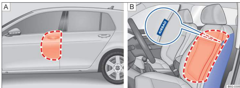
Fig. 36 On the driver side. A: Location and deployment zone of the side airbags. B: Location and deployment zone of the side airbags in the padding on the outboard side of the front seat backrests.
