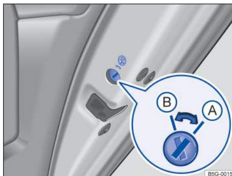
Fig. 58 In the rear passenger side door: Child safety lock (A) deactivated, (B) activated.
