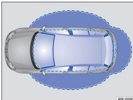
Fig. 50 Ranges of the Keyless Access system. Outside the vehicle: Unlocking range. Inside the vehicle: Starting range.
