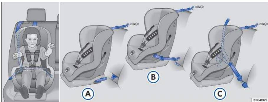
Fig. 41 All convertible child restraints have lower anchors and a top tether. Figures (A) and (B) show how to correctly install a LATCH/UAS seat. Figure (C) shows the set up of a seat using the vehicle's safety belt system.
