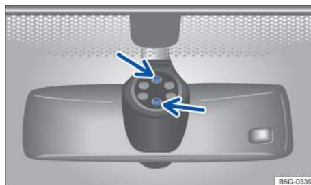
Fig. 83 Inside the front windshield above the inside mirror: Sensitive rain sensor surface (arrows).
