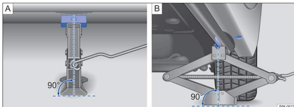
Fig. 190 Jack in position at the left rear lift point.
