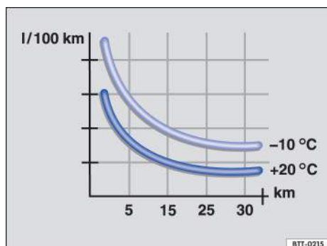
Fig. 94 Fuel consumption in l/100 km at two different outside air temperatures.
