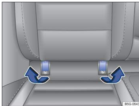
Fig. 43 On the rear outboard seat backrests: Removing the covers (if equipped) on the LATCH/UAS lower universal anchorages.
