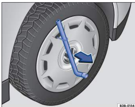
Fig. 183 Pulling the wheel cover off.
