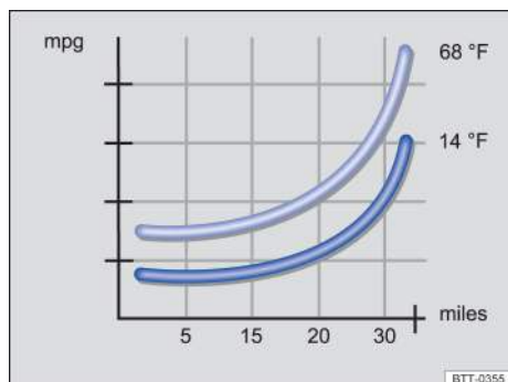
Fig. 93 Fuel consumption in miles per gallon (mpg) at two different outside air temperatures.
