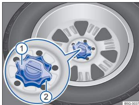
Fig. 178 In the luggage compartment: Handwheel holding the spare wheel in place (if equipped).
