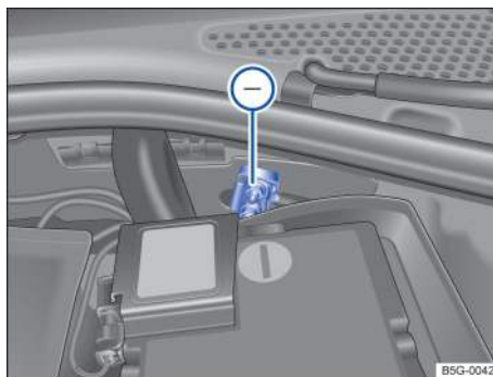
Fig. 160 In the engine compartment: Negative jump-start terminal ⊖.
