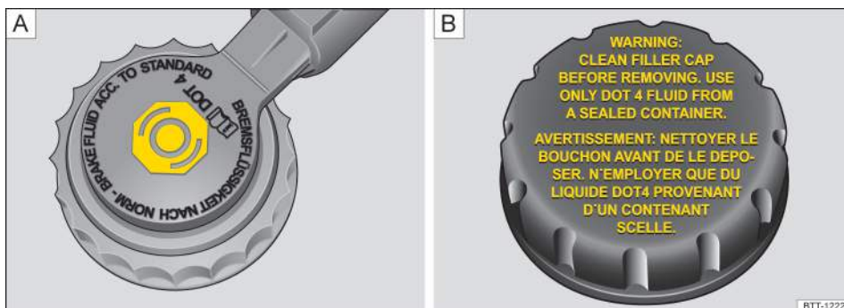
Fig. 174 In the engine compartment: Brake fluid reservoir cap (cap design may vary depending on vehicle equipment).
