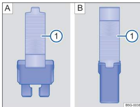
Fig. 159 Removing or installing a blade fuse with the plastic tweezers: A : Blade fuse. B : JCASE® fuse.
