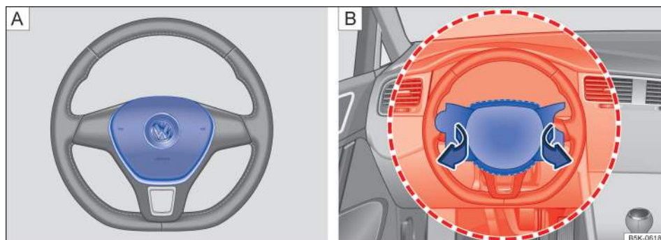
Fig. 34 Location and deployment zone of the driver front airbag.
