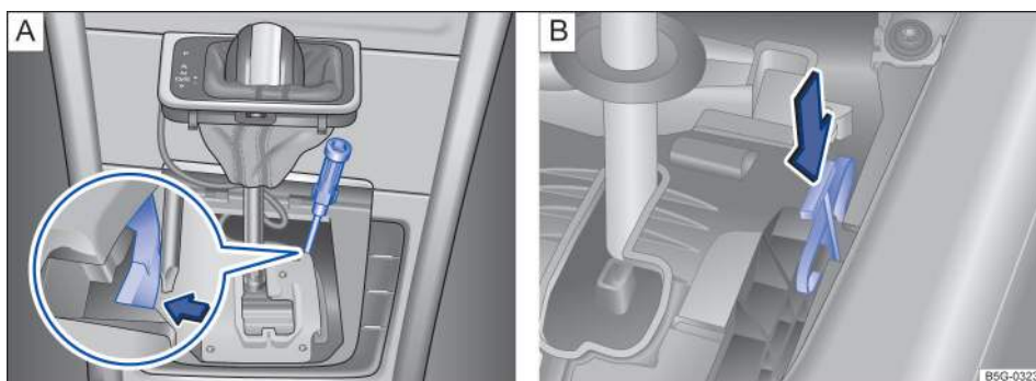
Fig. 105 Releasing the selector lever lock (versions A and B ).
