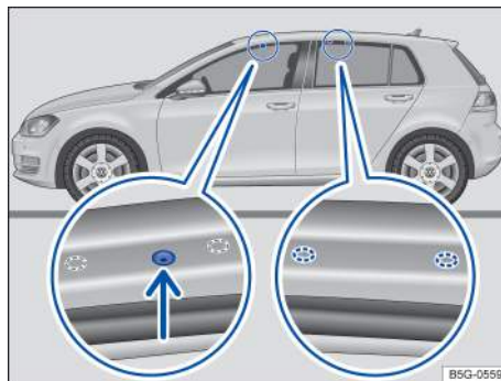
Fig. 149 Mounting points for the base carrier and roof rack.
