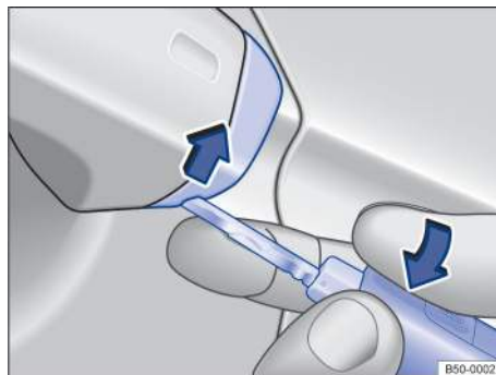
Fig. 54 Driver door handle: Removing the lock cylinder cover.
