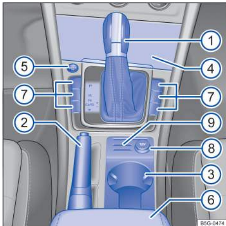
Fig. 8 Overview of the lower center console.
