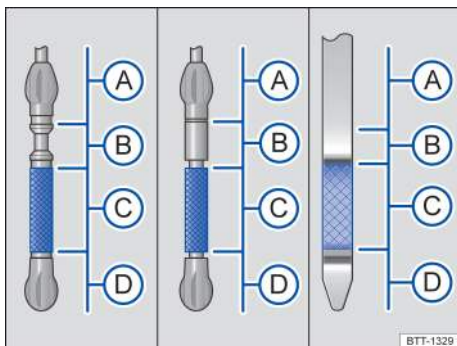
Fig. 170 Engine oil dipstick with oil level marks.
