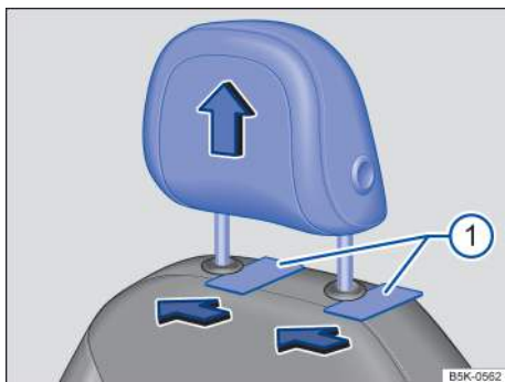
Fig. 72 Removing the front head restraints.
