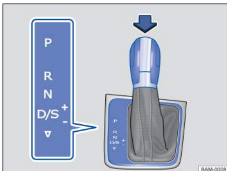
Fig. 101 Automatic or DSG transmission selector lever with shift lever release button (arrow).
