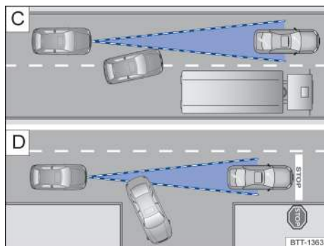
Fig. 109 C Vehicle changing lanes. D A turning and a stationary vehicle ahead.
