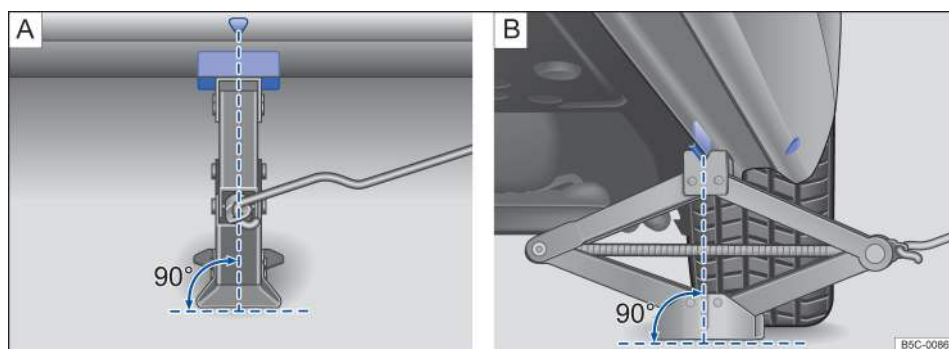
Fig. 188 Jack in position at the left rear lift point.
