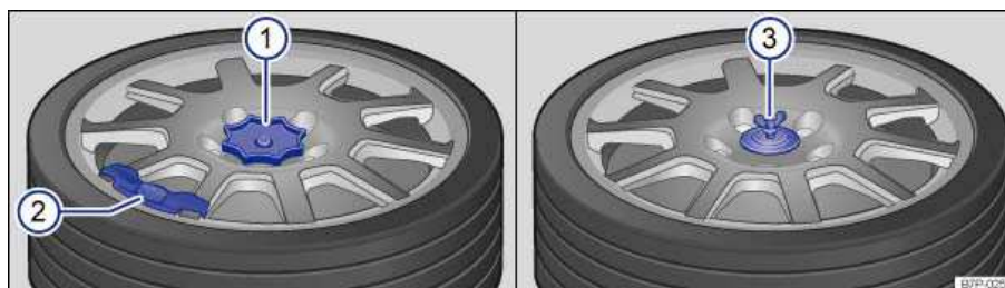
Fig. 113 Under the luggage compartment floor panel: Collapsible spare tire with threaded retainer (left) and collapsible spare tire with fastening bolt and washer (right).
