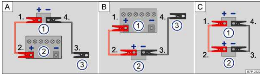
Fig. 350 The jumper cables are attached according to diagram A, B or C depending on how the vehicle is equipped.
