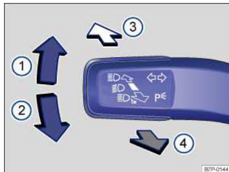
Fig. 84 Turn signal lever and high beam switch.
