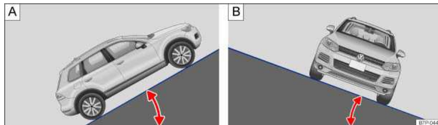
Fig. 310 Illustration of grade (gradient angle) A and lateral angle B.
