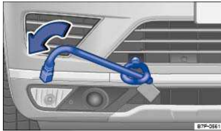
Fig. 352 In right front bumper: Screwing in towing eye.
