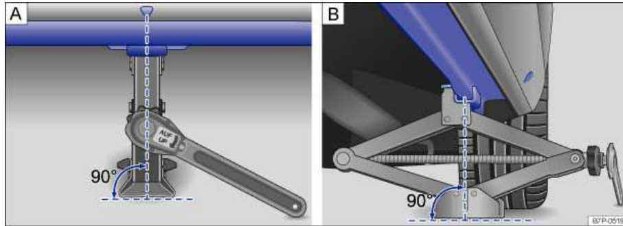
Fig. 341 Jack in position at the left rear lift point.
