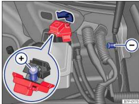
Fig. 344 In the engine compartment: Compressor connection terminals.
