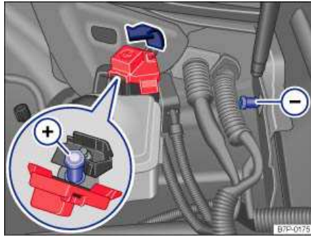
Fig. 349 In the engine compartment: Positive jump-start terminal + and negative jump-start terminal -.
