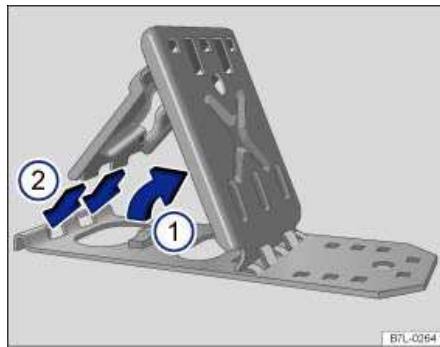
Fig. 335 Setting up folding chock.
