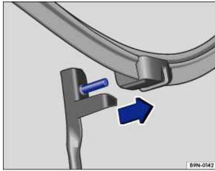
Fig. 321 Changing the windshield wiper blades.
