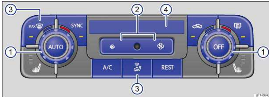
Fig. 301 In the front center console: Climatronic controls.
