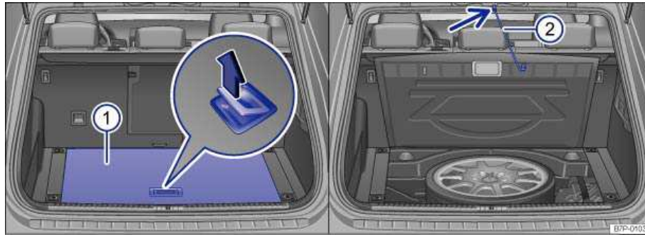
Fig. 106 In the luggage compartment: Lifting luggage compartment floor panel and securing it with retaining strap.
