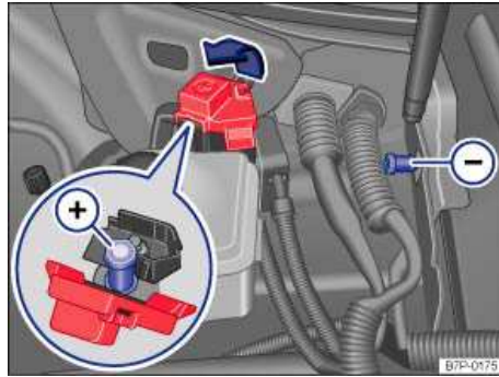
Fig. 114 Connection points in the engine compartment for the collapsible spare tire compressor.
