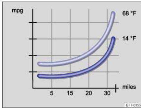
Fig. 255 Fuel consumption at 2 different outside air temperatures.
