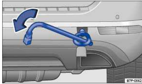
Fig. 353 In right rear bumper: Screwing in towing eye.
