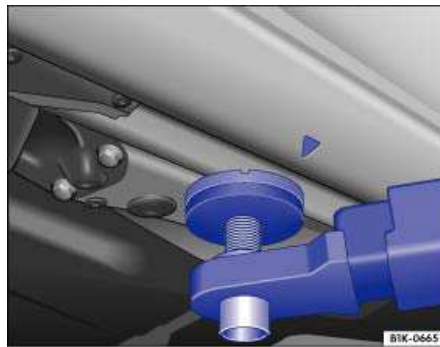
Fig. 151 Rear lift point for workshop hoist or floor jack.
