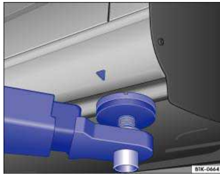
Fig. 150 Front lift point for workshop hoist or floor jack.
