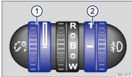
Fig. 74 To the left of the steering wheel: Thumbwheel to adjust instrument panel lighting 1 and headlight range adjustment 2 (if equipped).
