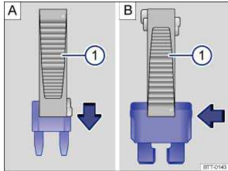
Fig. 172 Removing or installing a blade fuse with the plastic tweezers: A: MINI. B: ATO.
