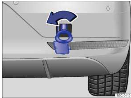
Fig. 179 In the right rear bumper: Installing the towing eye.
