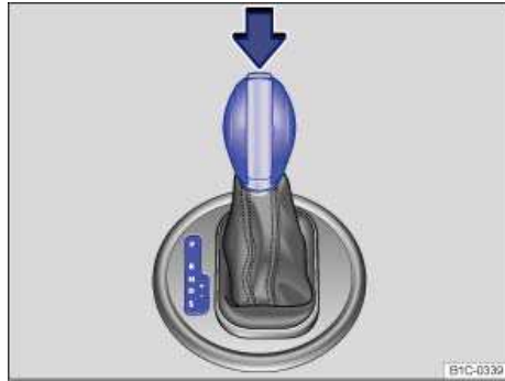
Fig. 119 Automatic transmission selector lever with shift lever release button (arrow).
