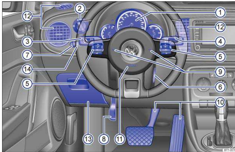
Fig. 6 Driver side overview.
