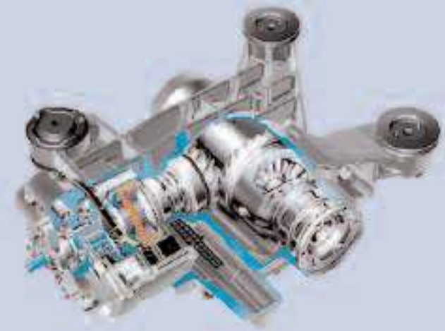
4MOTION all-wheel-drive system (detail)
