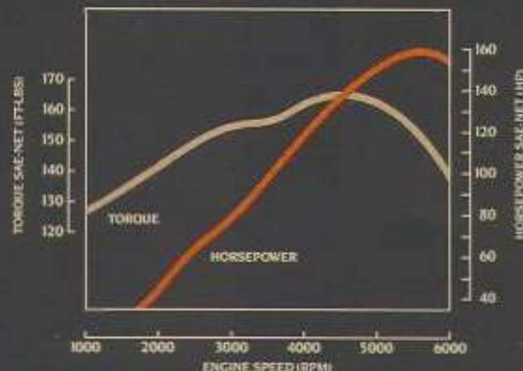
5M-GE TWIN CAM ENGINE MAP
