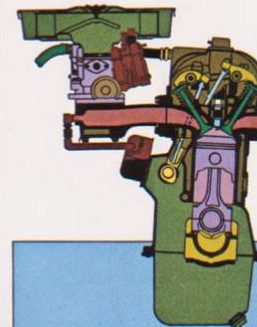
1588cc HEMI-HEAD ENGINE. ALL 1600 MODELS.
