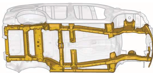
LADDER FRAME
