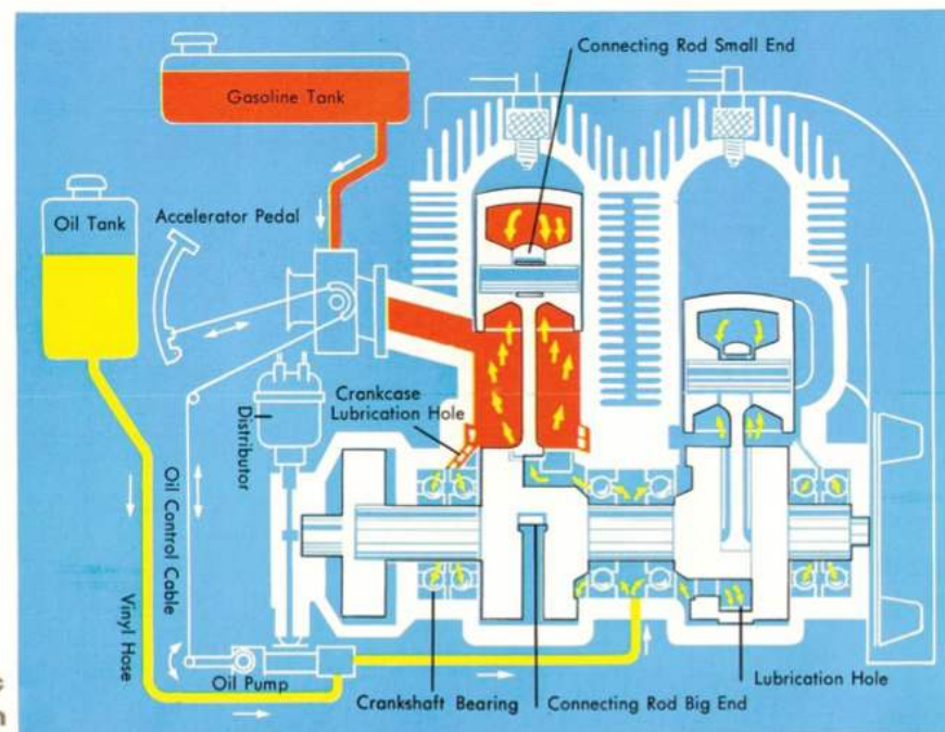
Subarumatic Lubrication Diagram
