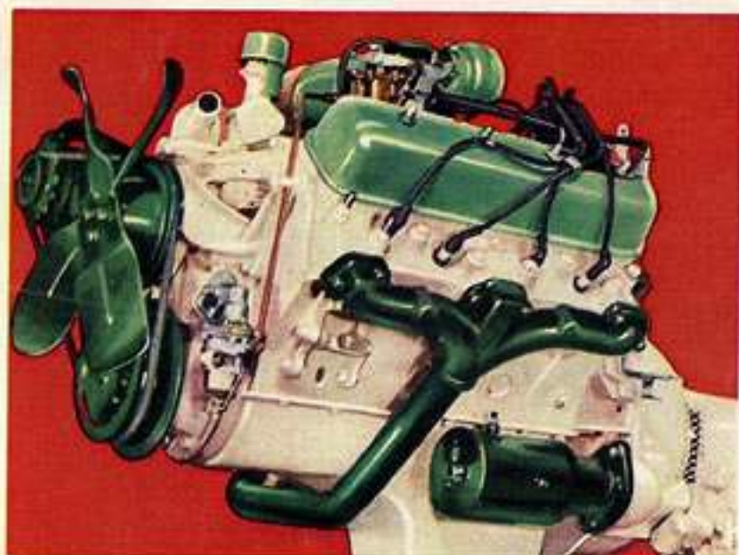
The new Commander V-8 "Pace-setter" engine
