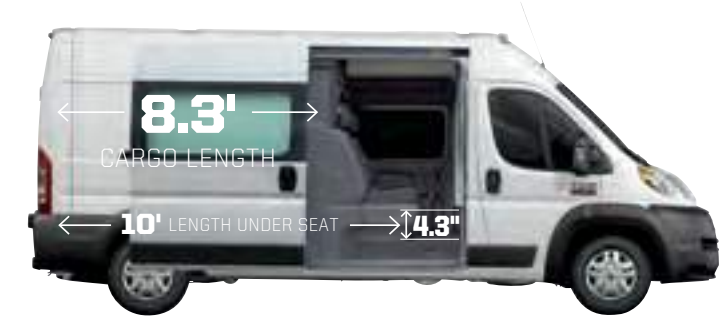
159-inch wheelbase with Crew Van Package
