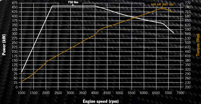
911 Turbo S Exclusive Series: 750 Nm between 2,250 and 4,000 rpm, 446 kW (607 hp) at 6,750 rpm
