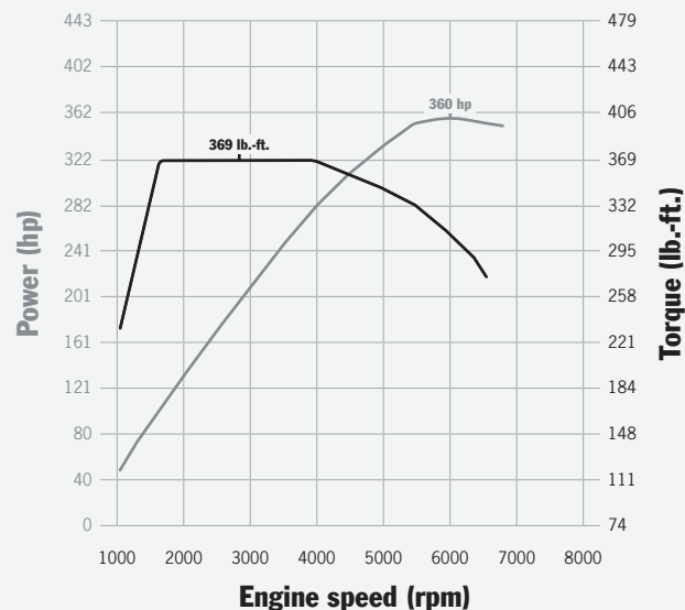
Macan GTS: 369 lb.-ft. at 1650–4000 rpm, 360 horsepower at 6000 rpm
