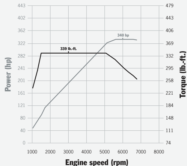
Macan S: 339 lb.-ft. at 1450–5000 rpm, 340 horsepower at 5500–6500 rpm
