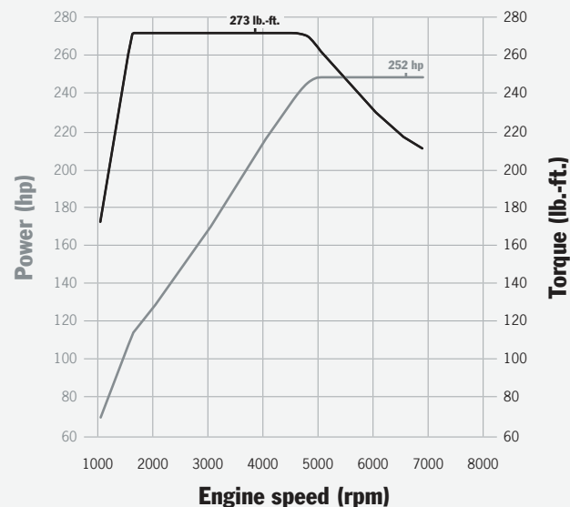
Macan: 273 lb.-ft. at 1600–4500 rpm, 252 horsepower at 5000–6800 rpm
