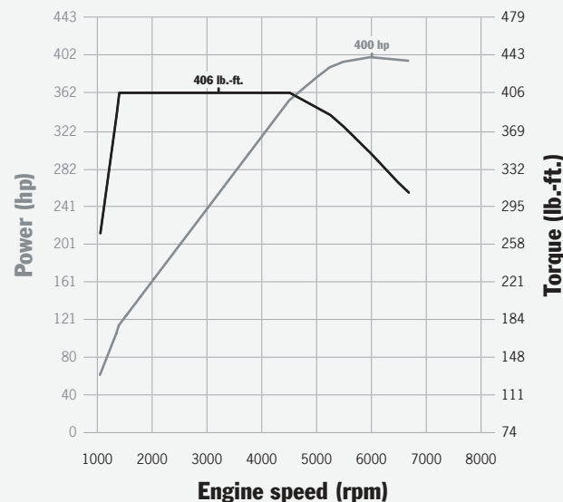
Macan Turbo: 406 lb.-ft. at 1350–4500 rpm, 400 horsepower at 6000 rpm
