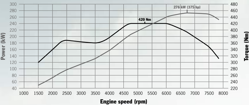
Boxster Spyder: 276 kW (375 hp) at 6,700 rpm, 420 Nm between 4,750 and 6,000 rpm
