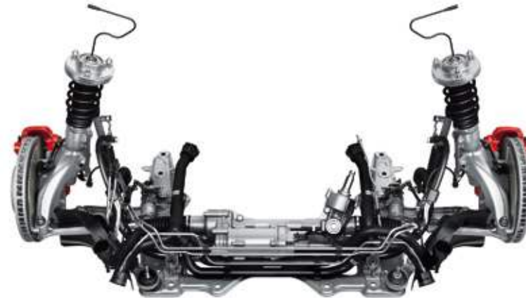
Front axle of the 911 Carrera S
