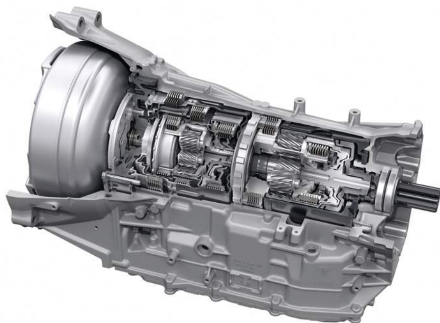
8-speed Tiptronic S gearbox
