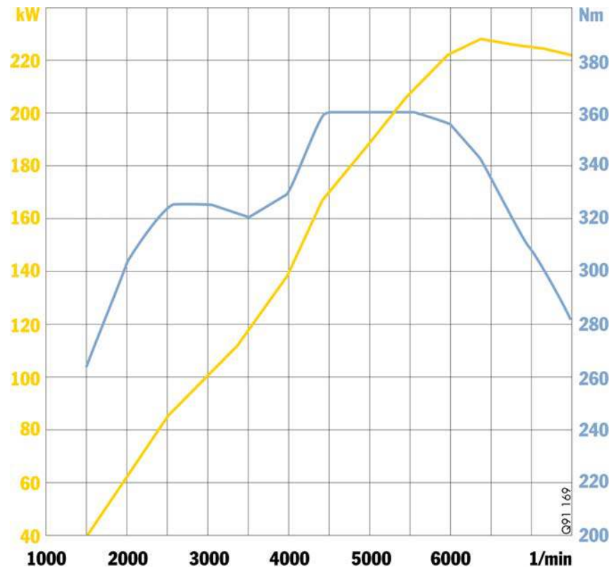
Engine diagram at full power, Boxster S
