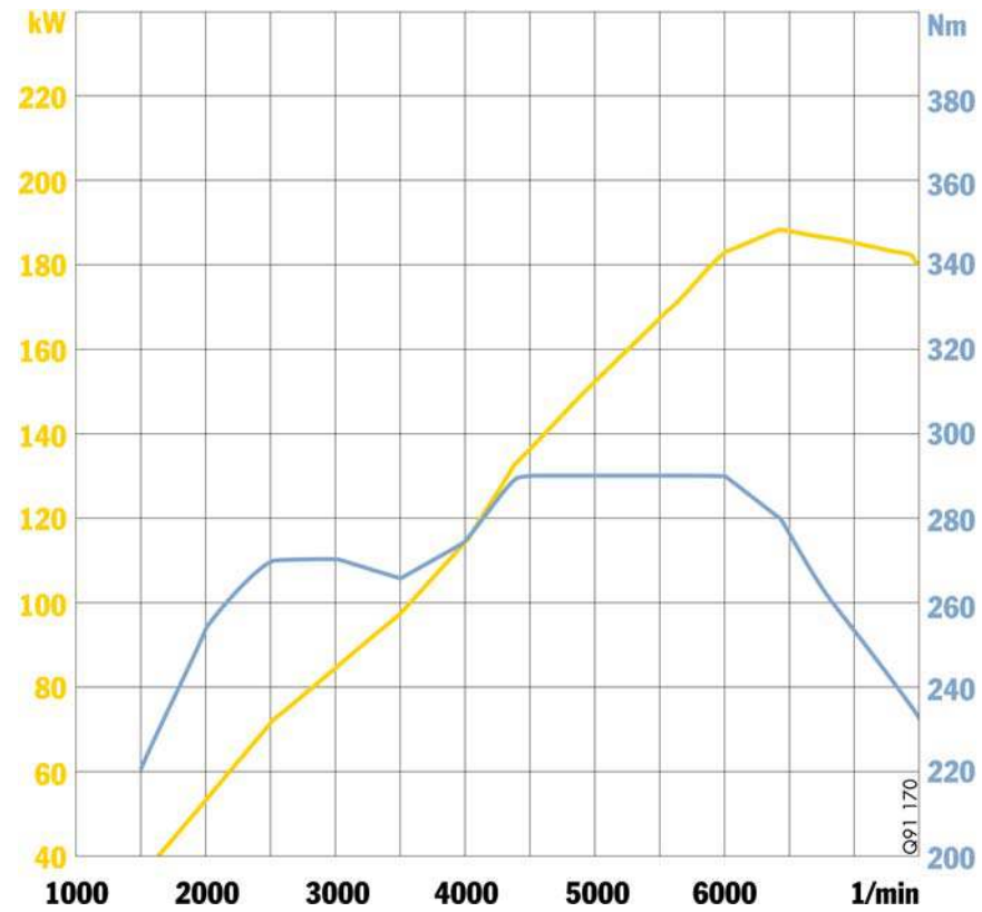
Engine diagram at full power, Boxster
