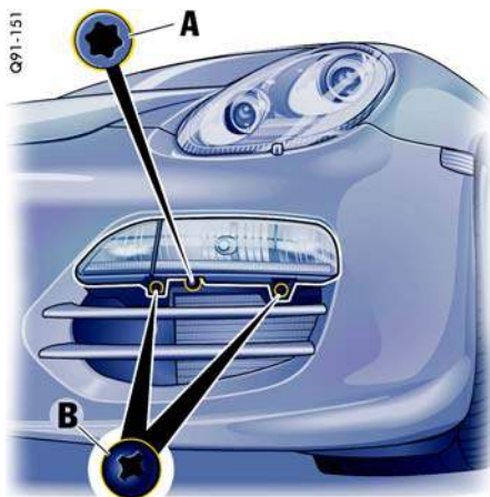
A - Fog light height adjustment B - Fastening screws
