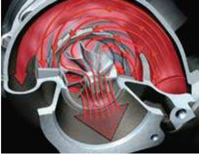
Guide vanes closed
