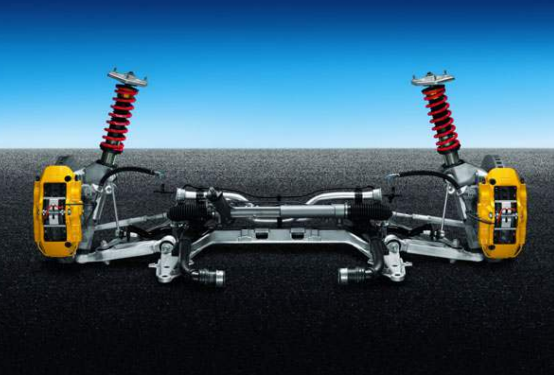
Front axle with Porsche Ceramic Composite Brake (PCCB)
