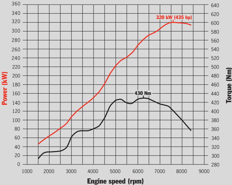
911 GT3: 430 Nm at 6,250 rpm, 320 kW (435 hp) at 7,600 rpm
