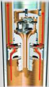
Left: Compression in 'Normal' mode – damper piston and bypass valve Right: Compression in 'Sport' mode – damper piston only
