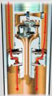
Left: Rebound in 'Normal' mode – damper piston and bypass valve Right: Rebound in 'Sport' mode – damper piston only
