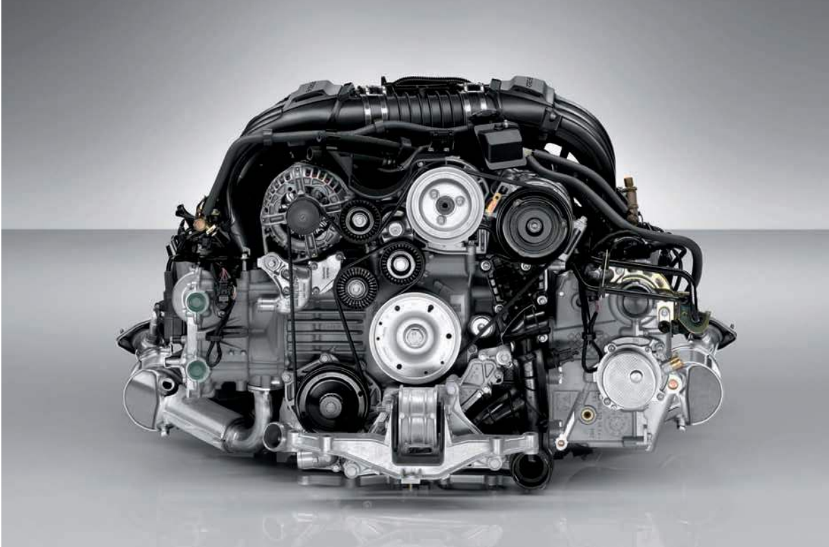
3.4-liter six-cylinder boxer engine
