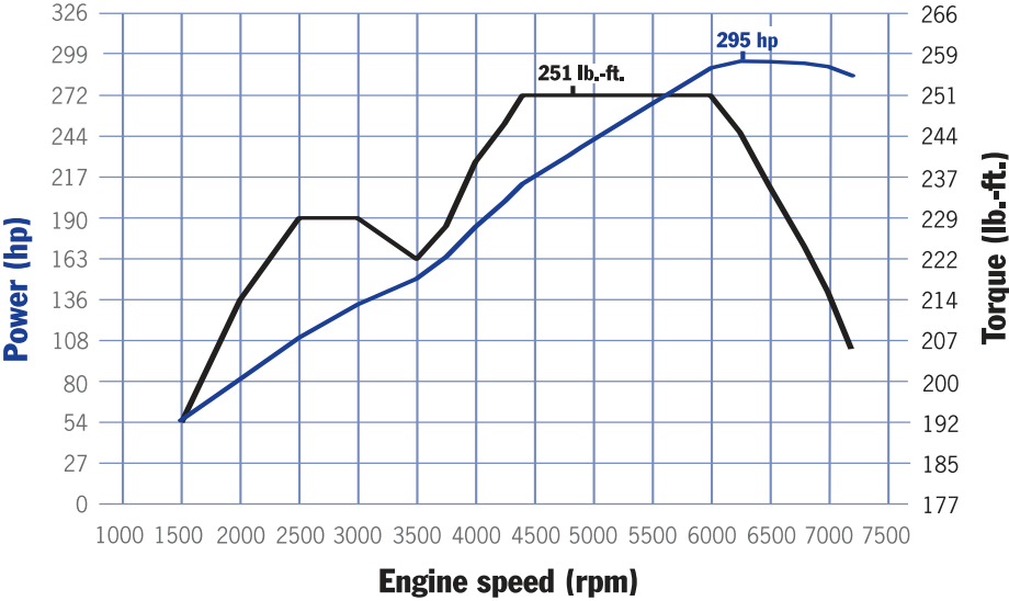
Cayman S: 251 lb.-ft. between 4400 and 6000 rpm, 295 horsepower at 6250 rpm
