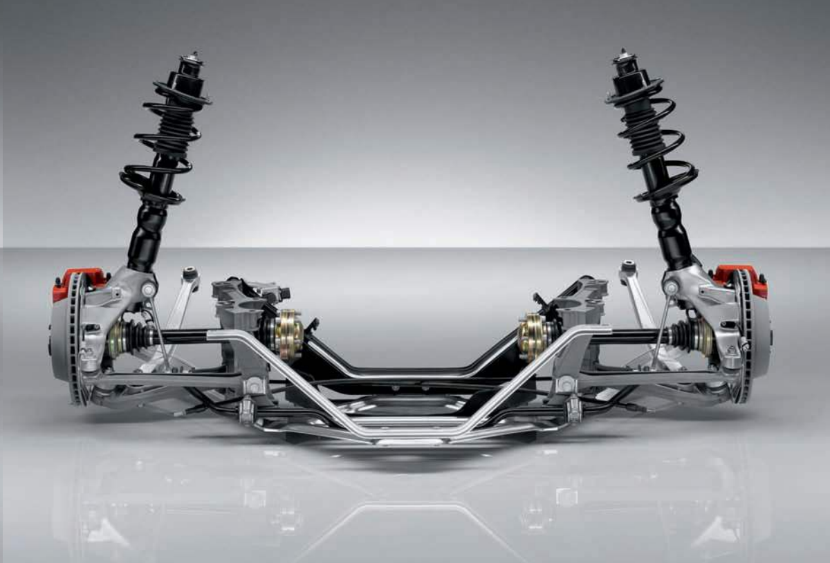
Rear axle with MacPherson struts and lateral control arms
