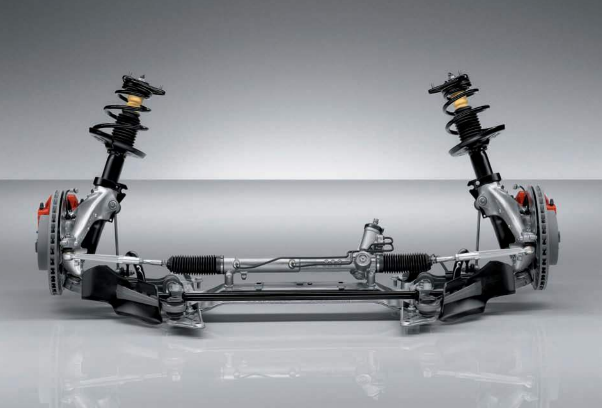
Front axle with MacPherson struts and lateral control arms
