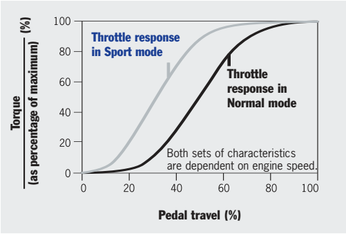
Comparison of throttle maps in Normal and Sport modes
