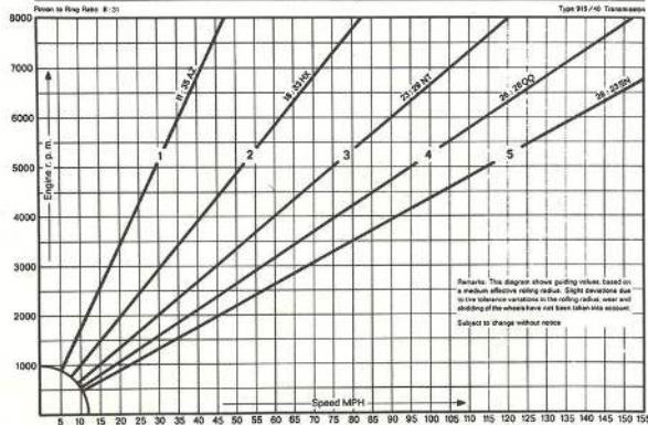
Transmission Diagram 911 S/Carrera 5-speed-transmission
