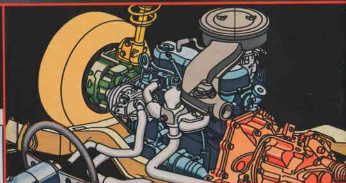
The Fiero engine/drivetrain cradle.
