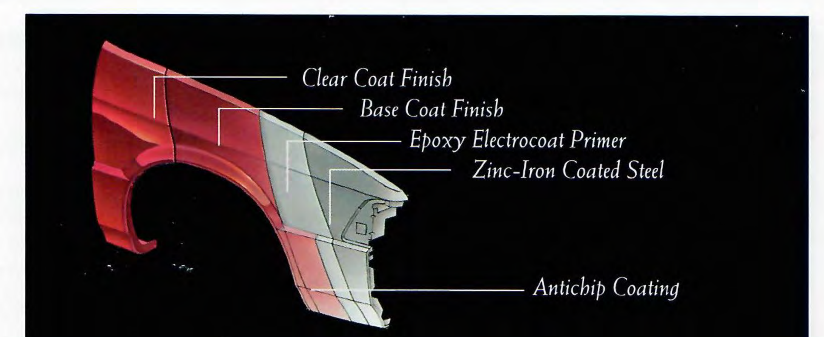
Anticorrosion protection: All body panels, except roof, are two-side galvanized/galvannealed, then three layers of primer, paint and clear antichip coatings are applied to create an environmentally resistant mirror finish.
