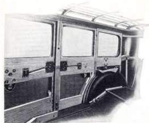
A solid hardwood frame, fully sheathed in metal panels—such is the make-up of every Oldsmobile Six body
