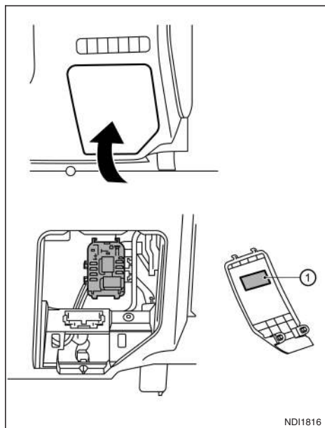
Secondary fuse box RHD models
