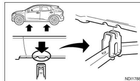
Jacking points
