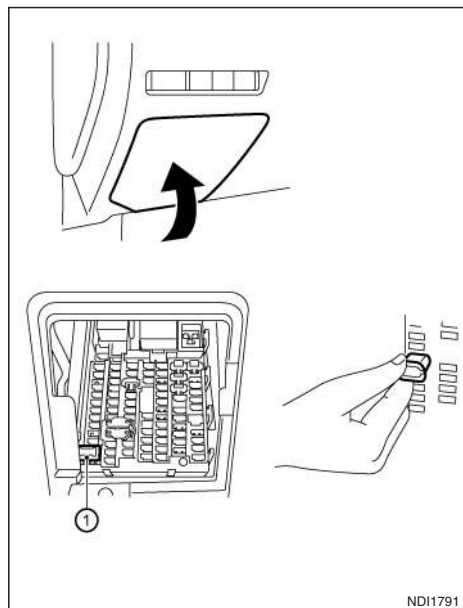
Primary fuse box LHD models
