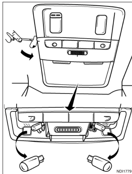
Room light/Map lights (where fitted)
