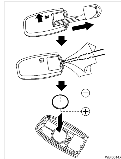
Intelligent Key
