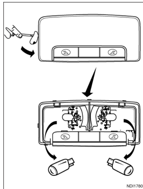
Room light – rear (where fitted)
