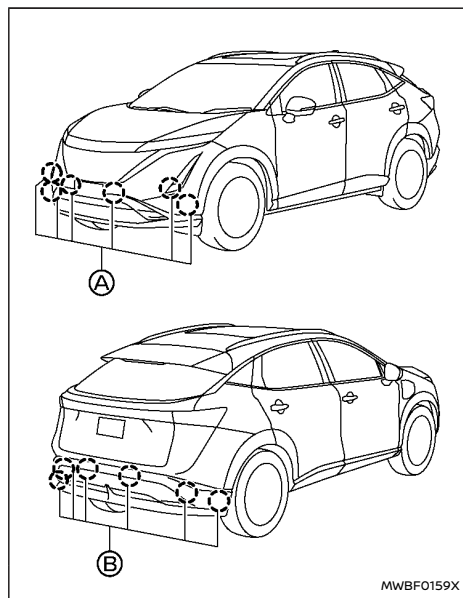
12 sensors
