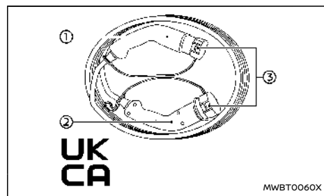
NISSAN Mode 3 cable (Type 2)
