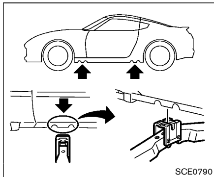
Jack-up point
