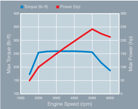
Output data according to new SAE spec 1349.
