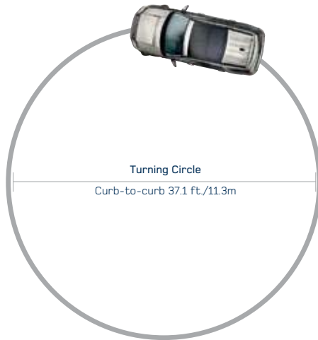
Vehicle Geometry
