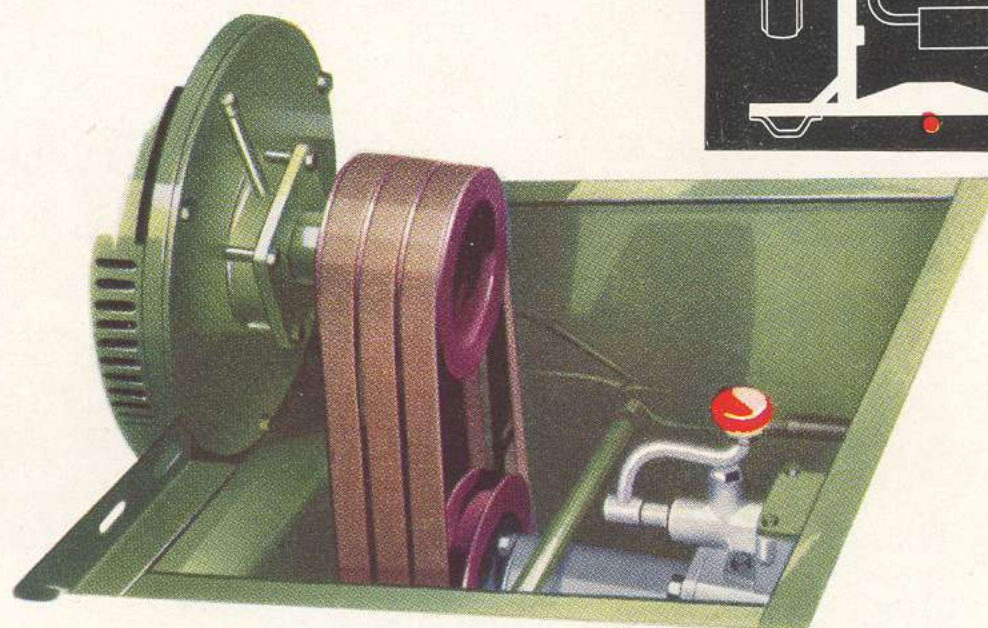
Showing the three-pulley drive of the centre power take-off unit in operation.
