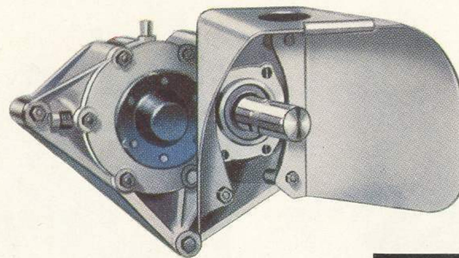
Rear power take-off drive section for operating, through a splined shaft, machinery towed by the vehicle.
