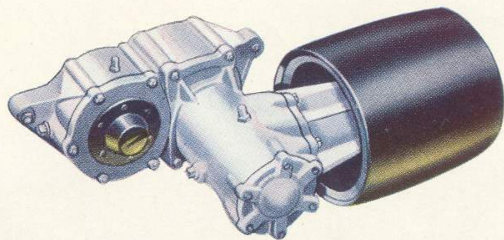
Rear power take-off pulley unit which provides a flat belt drive for standing machinery.
