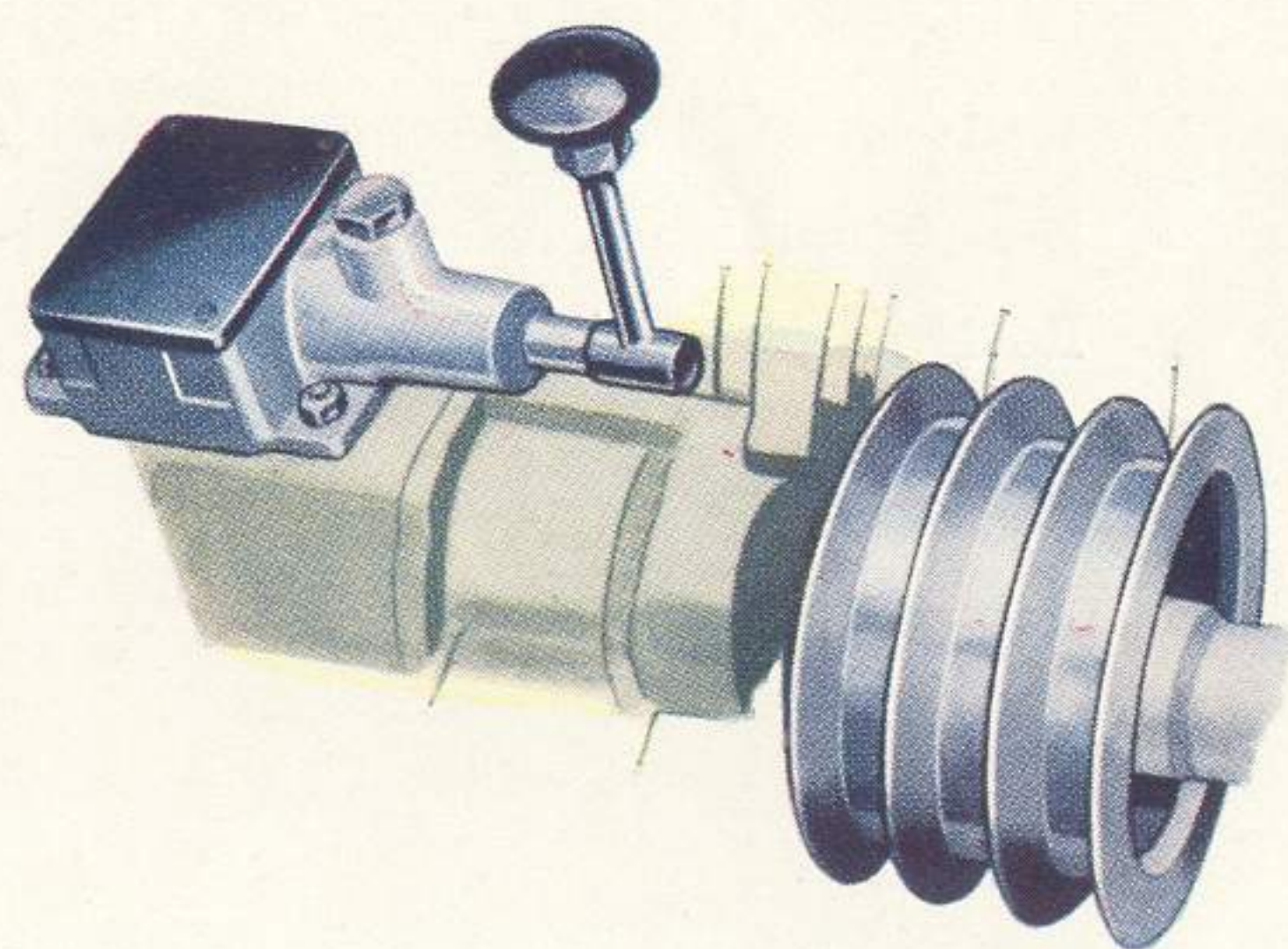
Centre power take-off may be used to operate an appliance mounted in the body of the vehicle.
