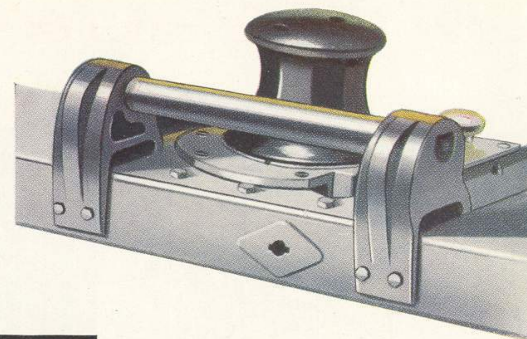
A capstan winch can be fitted to the front of the Land-Rover for recovery and haulage work.
