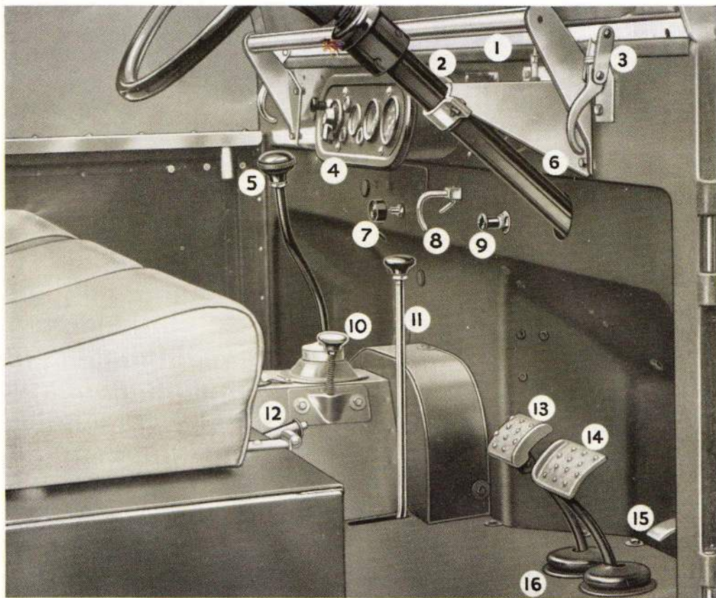
The forward compartment of the Land-Rover.
