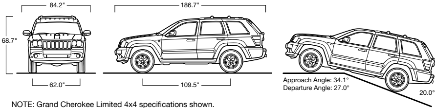
NOTE: Grand Cherokee Limited 4x4 specifications shown. Dimensions of SRT8®: overall length 195.1; track, front/rear 63.3/62.1; height 67.4.
