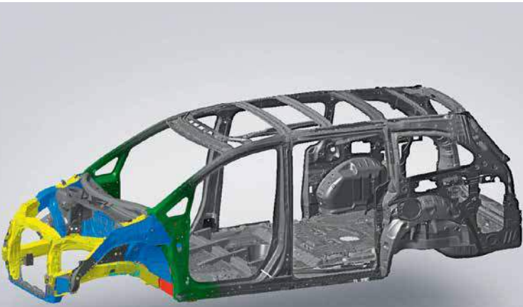
ACE BODY STRUCTURE
