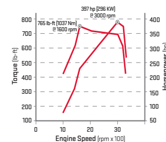
Duramax Diesel 6.6L V-8 Horsepower & Torque • SAE Certified
