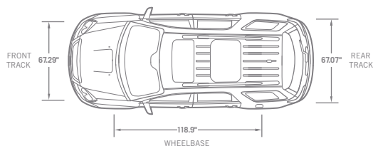
FIGURE 11: WIDE FRONT/REAR TRACKS/LONG WHEELBASE
