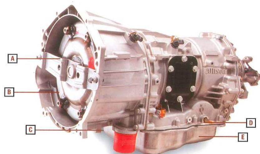
Allison 1000 Series Five-speed Automatic Transmission
