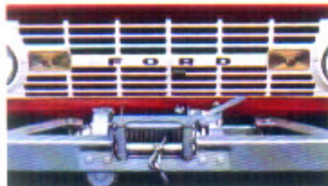
Front-Mounted Winch with 150 feet of 5/16-in. cable. A power take-off driven.
