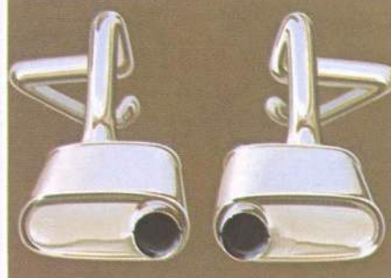
Dual resonator/tailpipe
