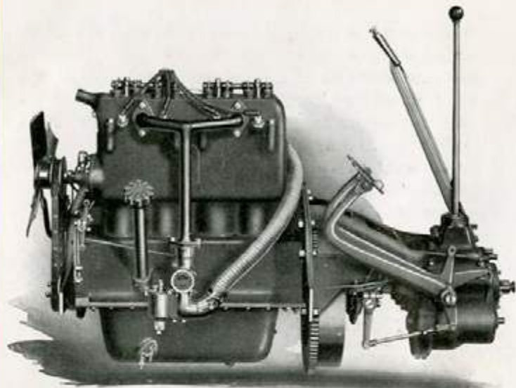
Left or intake side view of the Chevrolet Valve-in-head One-Ton Truck motor. Illustration shows the manifold, the carburetor and the transmission assembly of the unit type power plant.
