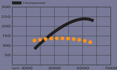
3.8L SUPERCHARGED V6
