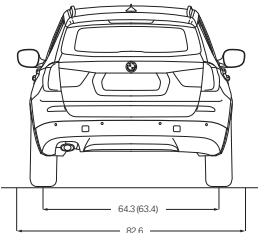
All dimensions in the technical drawings are given in inches. Figures in parentheses ( ) refer to the BMW X3 xDrive35i.
