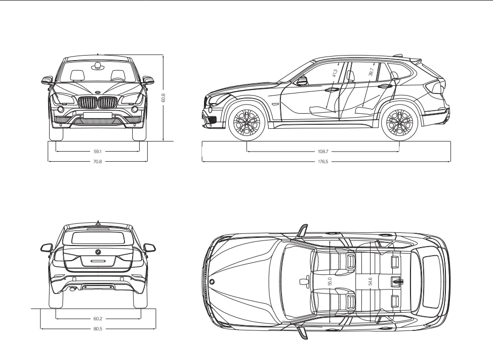
All dimensions in the technical drawings are given in inches.
