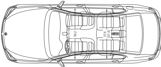
All dimensions of the technical drawings in inches and apply to all models. Figures in ( ) refer to the 7 Series "i" models where different; additional figures in [ ] refer to 740i, 750i and 750i xDrive where different.
