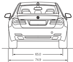
All dimensions of the technical drawings in inches and apply to all models. Figures in ( ) refer to the 7 Series "i" models where different; additional figures in [ ] refer to 740i, 750i and 750i xDrive where different.
