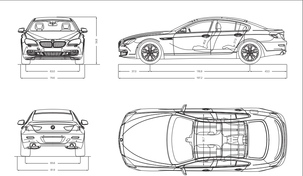
All dimensions in the technical drawings are given in inches.
