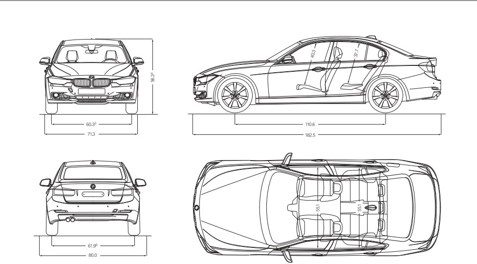
All dimensions in the technical drawings are shown, in inches, for 328i; dimensions for other models, if different, are footnoted.
