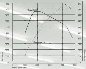
High performance, low emissions – the efficient engine of the X5 xDrive35d.
